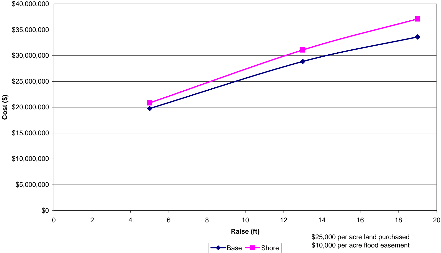
FIGURE 5.13 Union Reservoir Feasibility Study Estimated Construction, Engineering, and Land Costs
