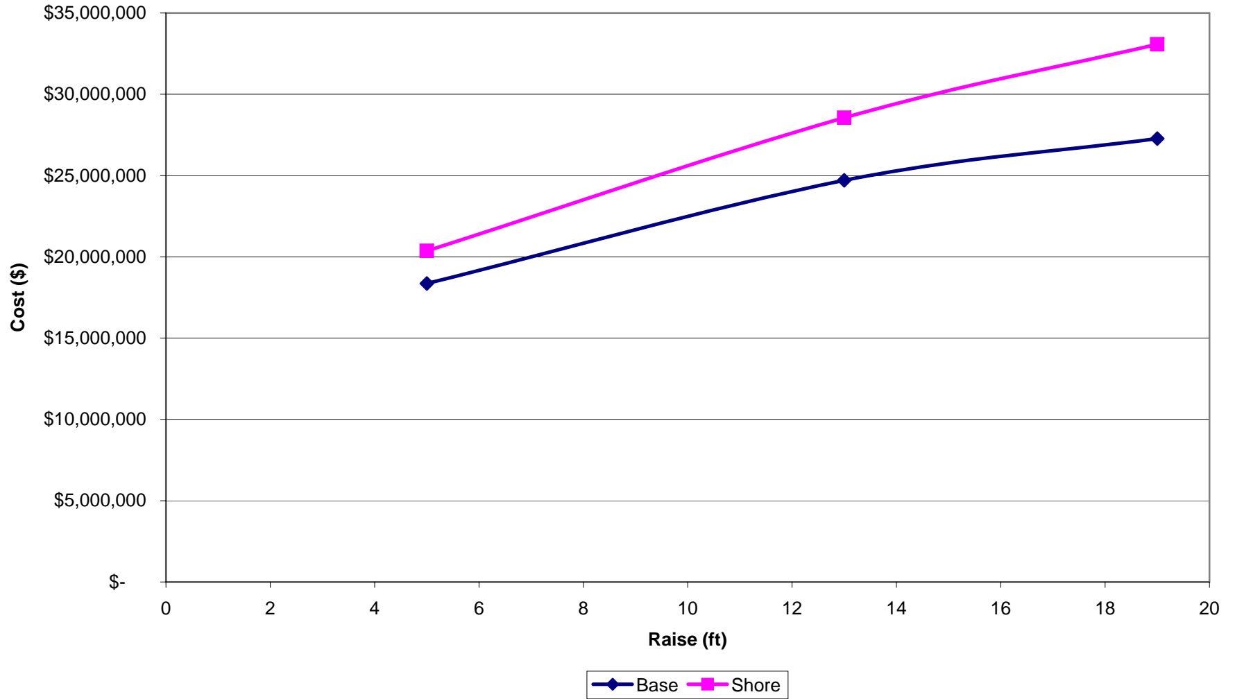
FIGURE 5.11 Union Reservoir Feasibility Study Estimated Construction & Engineering Costs
