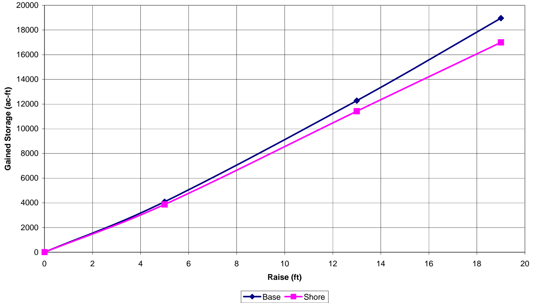
FIGURE 5.15 Union Reservoir Feasibility Study Gained Storage
