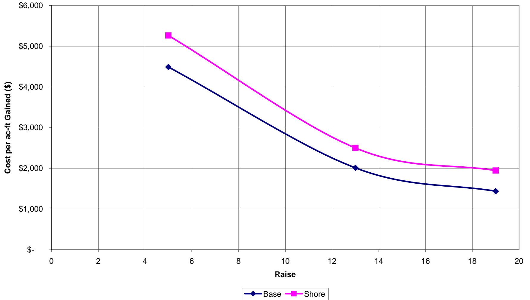
FIGURE 5.12 Union Reservoir Feasibility Study Estimated Construction & Engineering Cost Per Acre-ft Gained
