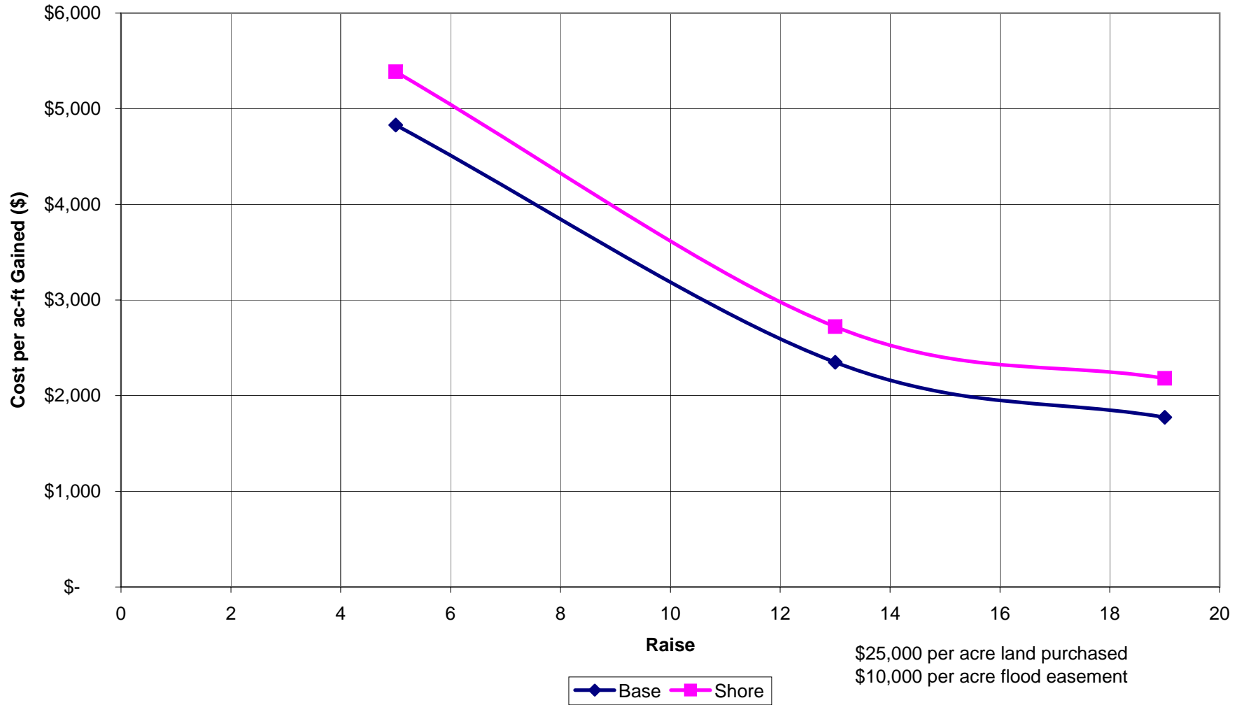
FIGURE 5.14 Union Reservoir Feasibility Study Estimated Construction, Engineering, and Land Cost Per Acre-ft Gained
